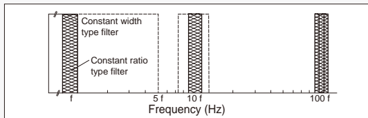
Fig. 2 Bandwidth representation for constant ratio and constant width filter on logarithmic scale
