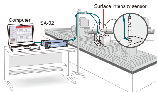
Connection example
