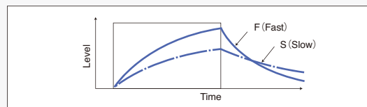
Fig. 4 Time weightings of sound level meters
